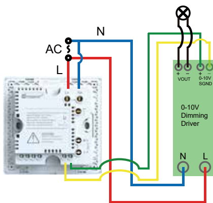
Connection 1: 0-10V Dimming
