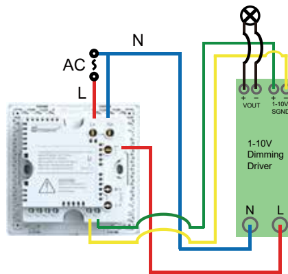
Connection 2: 1-10V Dimming
